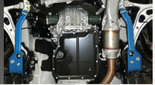
Power Brace - Front Side : 6A5 492 FS - $227 msrp
