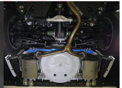
Power Brace - Rear Member : 6A1 492 RM - $227 msrp
