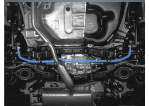
Rear Sway Bar : 24mm / Solid <for 2 WD> <for 4 WD> - 1A1 311 B24 - 1A2 311 B24 - $347 MSRP - $347 MSRP - 4996 3380 62246 - 4996 3380 62253
