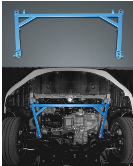
Power Brace : Front - 1A1 492 F - $307 MSRP - 4996 3380 48516
