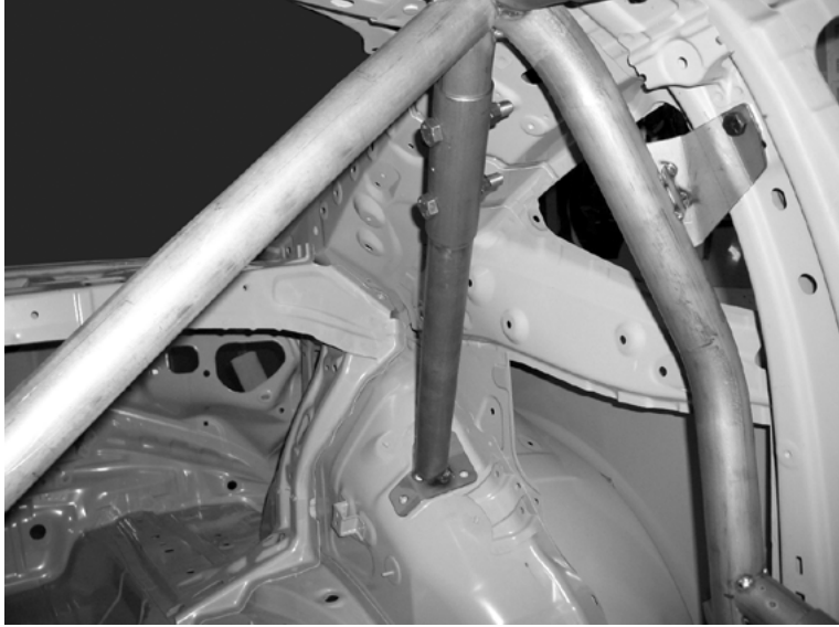
Rear Bar - Left Installation
