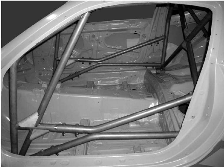
Side Door Bars Installation
