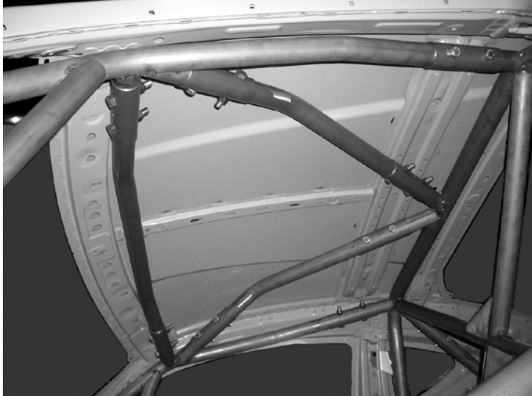
Roof Bars Installation
